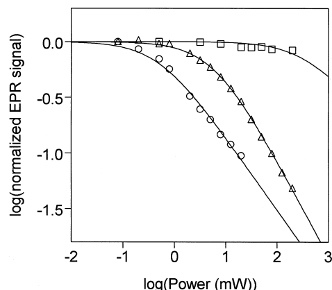
Fig. 4. Saturation plot of P. furiosus GAPOR W^{5+} and [4Fe-4S]^{+} S = 1/2 signals at 19 K. Trace A, [4Fe-4S]^{+} S = 1/2 signal ( \square ). Trace B, W_1^{5+} signal ( \Delta ). Trace C, W_2^{5+} signal ( \circ ). Normalized EPR signal \equiv (signal/ \sqrt{\text{power}} )/(low-power signal/ \sqrt{\text{low-power}} ).
