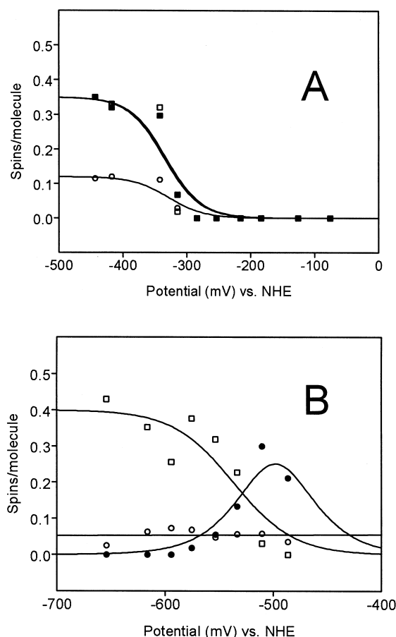
Fig. 5. Redox titrations of P. furiosus GAPOR. Dye-mediated redox titration (A) and GAP/3PG redox titration (B). The [4Fe-4S]^{1+} S = 3/2 signal ( \blacksquare ) is monitored at g = 5.22 with the EPR conditions as in the legend to Fig. 2. The [4Fe-4S]^{1+} S = 1/2 signal ( \square ) is monitored as the amplitude at g_y = 1.890 with the same EPR conditions. The W_1^{5+} signal ( \bullet ) is monitored at g_z = 1.923 and the W_2^{5+} signal ( \circ ) is monitored at g_z = 1.948 at 40 K with EPR conditions as in the legend to Fig. 1. The solid lines are fits for n = 1 redox transitions with the midpoint potentials given in Table 2.
